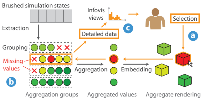
Fig. 8. The selection mechanism. The black arrows describe the flow of aggregation, while the orange arrows pointing in the opposite direction describe selection. The selected elements are depicted with an orange border.
