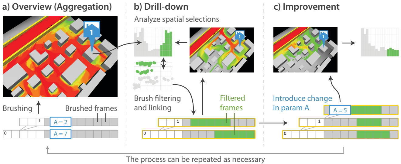
Fig. 2. The proposed solution for performing an analysis of an ensemble flooding simulation. a) The aggregations help the user understand what is happening in several selected simulation states (shown as dark grey) at once. b) When details are needed, selections (blue icon in the image) provide data to the information-visualization views. By brushing values of interest, the states associated with these values are highlighted, becoming green. c) The views allow the user to see the effects of any changes introduced. The user can continue filtering and introducing changes as necessary.
