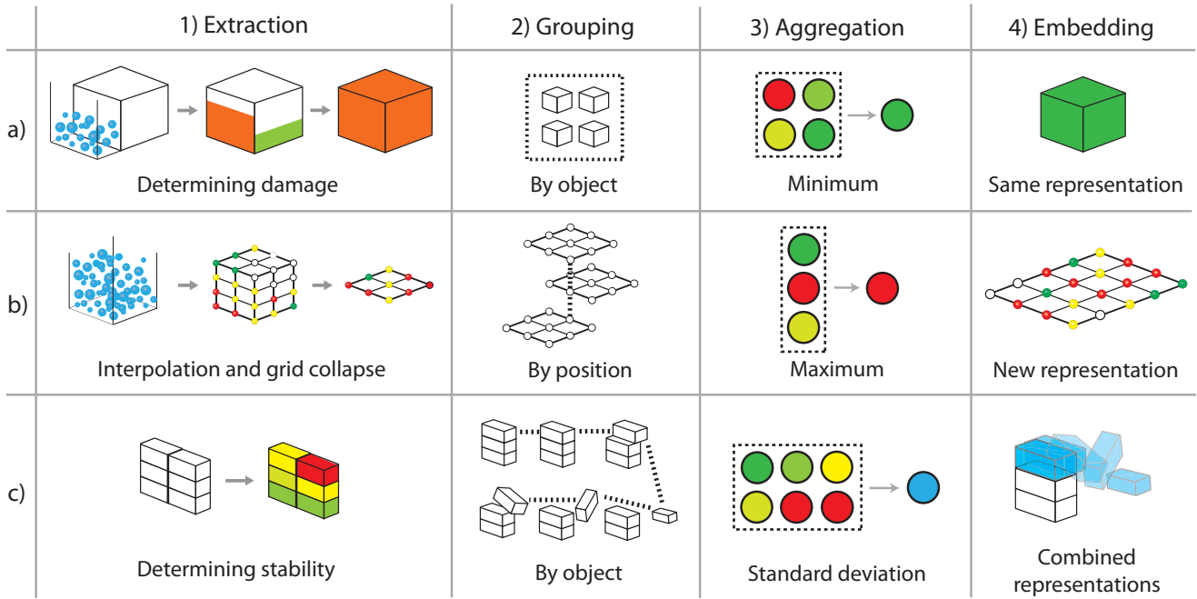
Fig. 3. The various types of aggregation: a) Object aggregation (buildings) b) Field aggregation (fluid) c) Instance aggregation (bags). The types of aggregation are shown progressing through the four phases of an aggregated rendering: 1) Extraction 2) Grouping 3) Aggregation 4) Embedding. The spectrum of colors from green to red indicates increasing values.
