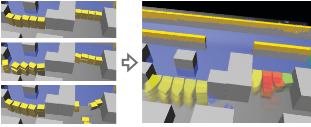
Fig. 6. Instance aggregation. Multiple states, three of which are shown to the left, are combined to create an aggregated rendering. The states are colored according to how much they've moved from their initial position, with red signifying the greatest movement.
