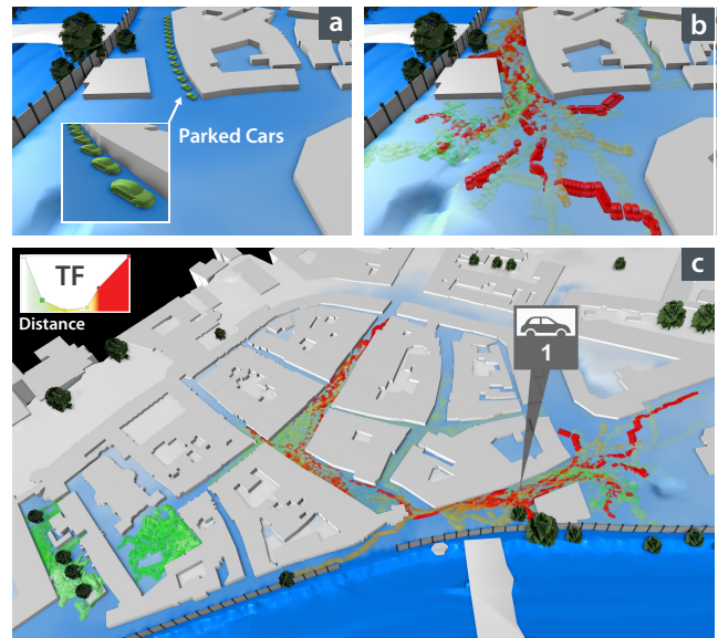
Fig. 12. Instance aggregation applied to cars. a) The initial state of the cars. b) A close-up of the car aggregation. The car positions are interpolated to compensate for the large time step size. c) An overview of the car movement. The cars on the left are mostly stationary, while the cars to the right move the most.
