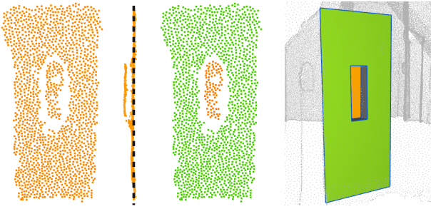
Fig. 2. The first step of the automatic reconstruction pipeline, a local RANSAC-based method, may capture nearby parallel structures (e.g. windows and facade) as a single segment (left). The least-median of squares method is used to fit a plane to the points of the dominant structure (middle left). By applying k-means clustering ( k = 2 ) (and subsequent automatic polygonalization and optimization) in the interactive modeling phase, a more detailed hierarchical reconstruction (middle right, right) is achieved.
