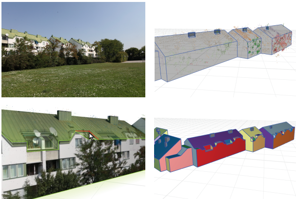
Fig. 12. Reconstruction of a building complex occluded by trees and bushes. Top left: An example photo of the data set. Top right: The segments extracted from the sparse point cloud (obtained from a photogrammetric approach) and the main structures after approximately three minutes of optimization-aided modeling. Bottom left: The reprojected images help the user to modify the polygon boundaries and to sketch new polygons forming the balconies. Bottom right: The final model after 20 minutes using the additional image information.
